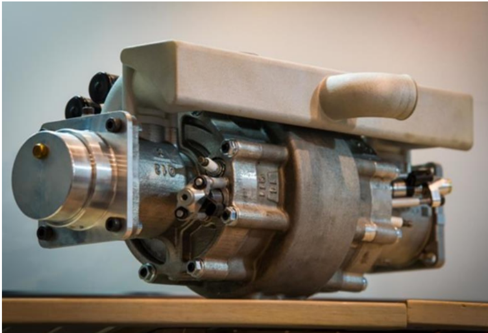
Figure 4 – le prototype Aquarius (2021)
